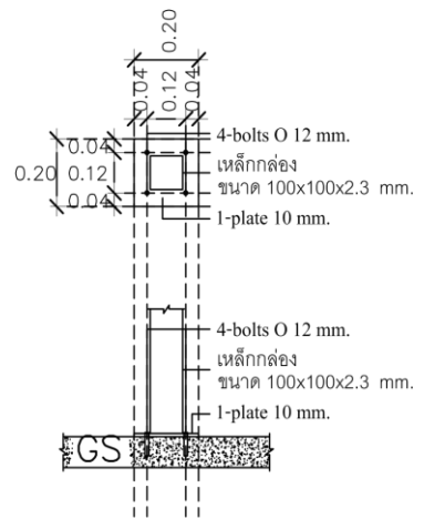
DETAIL CX
