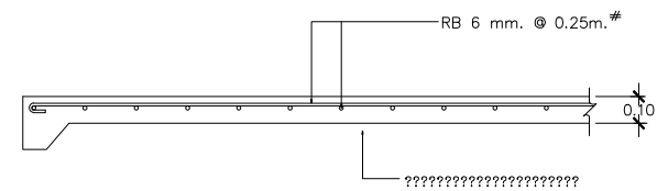
DETAIL GS
